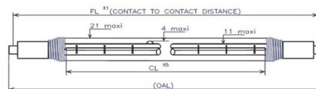
V Type (Jacketed emitter)
