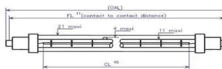
Vj Type (Jacketed emitter)
