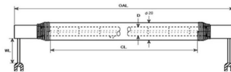
Bj Type (Jacketed emitter)
