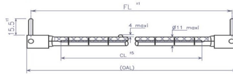
B Type (Jacketed emitter)
